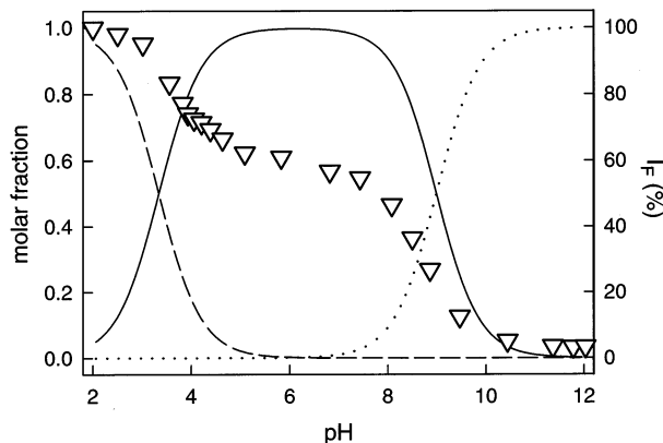
Fig. 4. pH dependance of the relative fluorescence intensity I_F of the anthracene fragment of the \text{Ni}^{\text{II}} scorpionate complex of ligand 6 (L) ( \nabla , right vertical axis) and distribution curves of the three species present at the equilibrium: [\text{Ni}^{\text{II}}(\text{LH}^+)]^{3+} , [\text{Ni}^{\text{II}}(\text{L})(\text{H}_2\text{O})]^{2+} , [\text{Ni}^{\text{II}}(\text{L})(\text{OH})]^+ (dashed, full and dotted line, respectively; left vertical axis).
